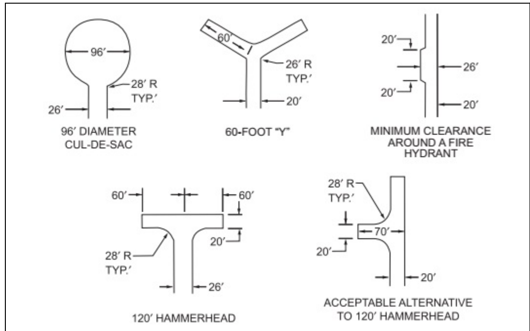
Figure 3-7a: Dead-End Fire Apparatus Access Road Turnaround
