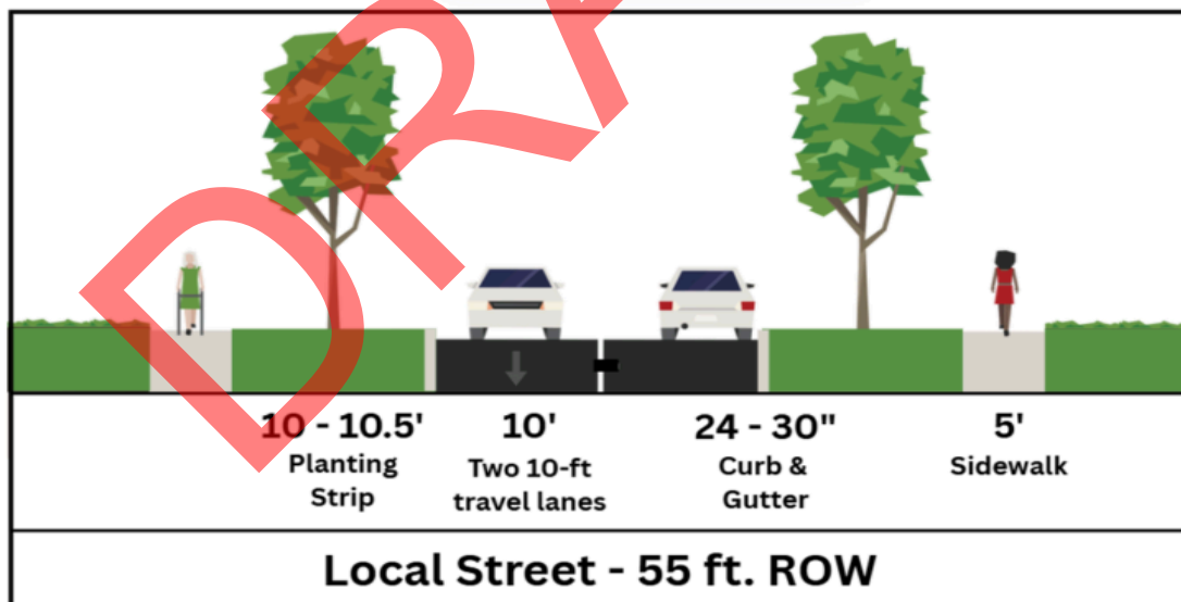
Figure 5.6 Street Tree Plantings (ROW width may vary)
